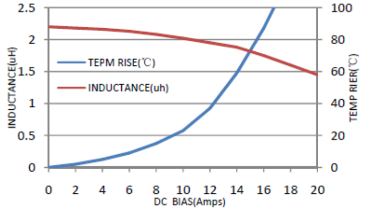
PIC10040Q-2R2M
