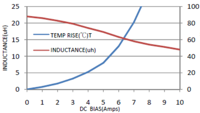
PIC10040Q-220M
