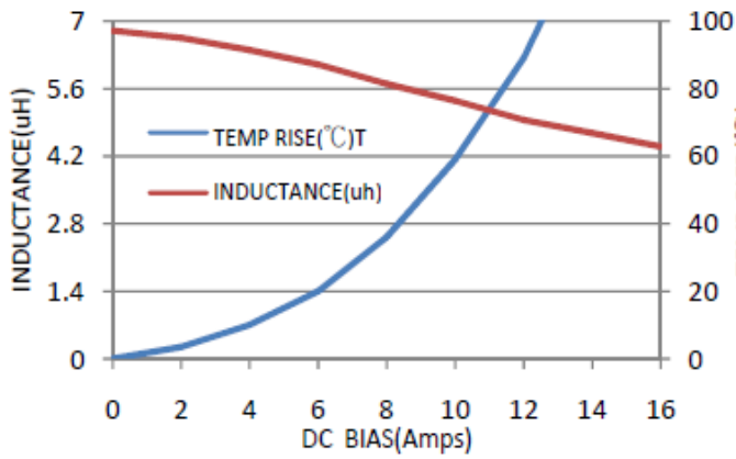
PIC10040Q-100M
