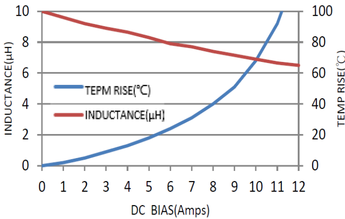
PIC10040Q-220M
