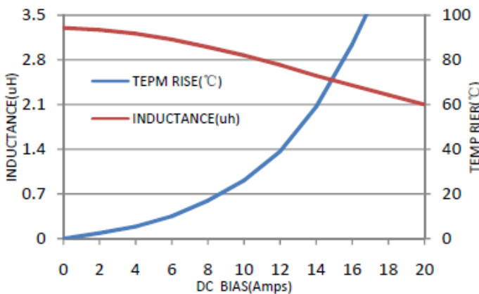
PIC10040Q-3R3M
