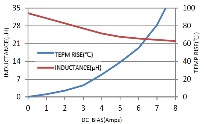
PIC10040Q-330M
