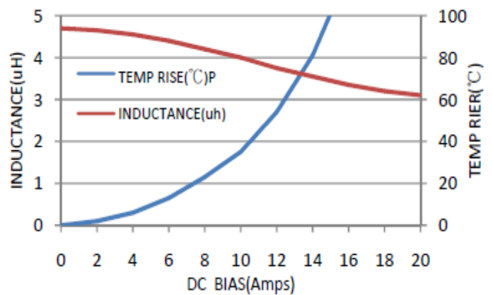
PIC10040Q-4R7M
