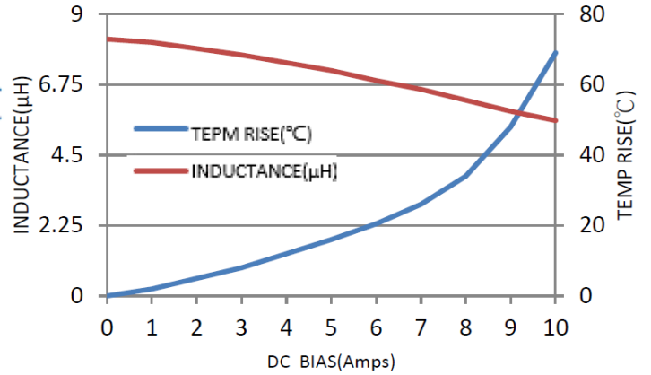
PIC10040Q-150M
