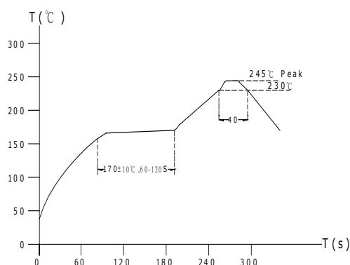
Lead-free the recommended reflow condition
