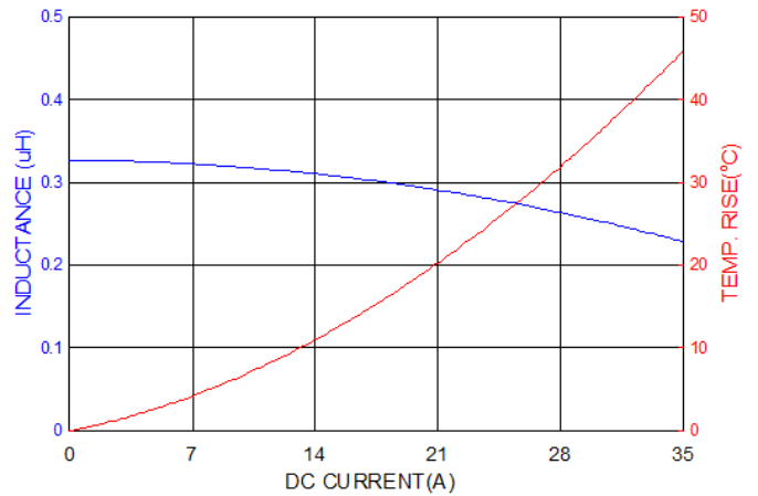
PIT07030A-1R0M
