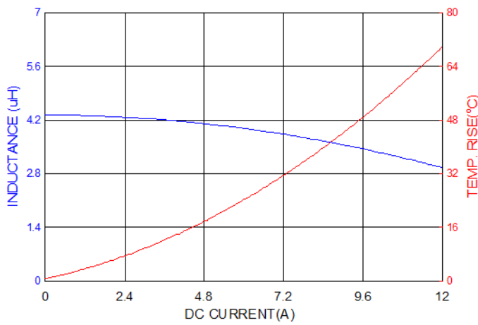
PIT07030A-4R5M
