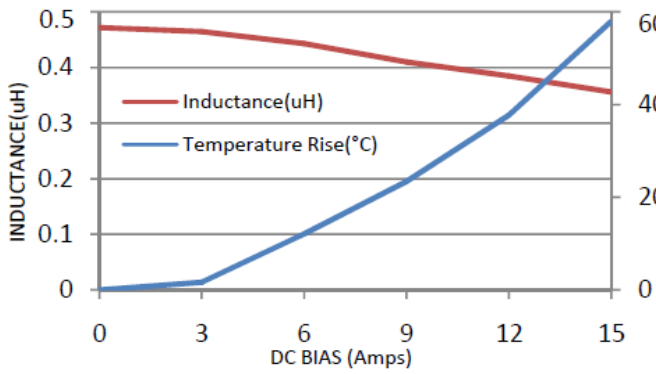
PIC05030-1R0M
