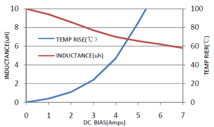
PIC05030-100M
