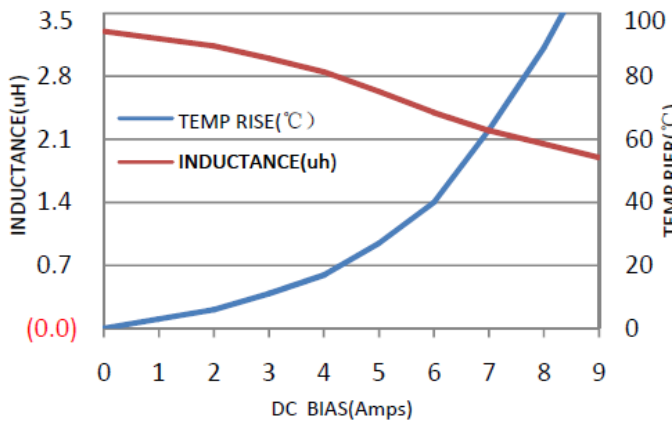
PIC05030-6R8M
