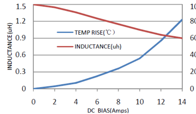
PIC05030-1R5M
