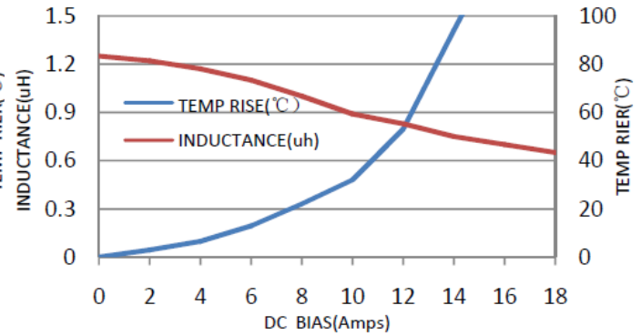
PIC05030-1R2M
