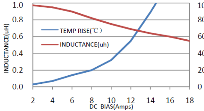
PIC05030-1R0M
