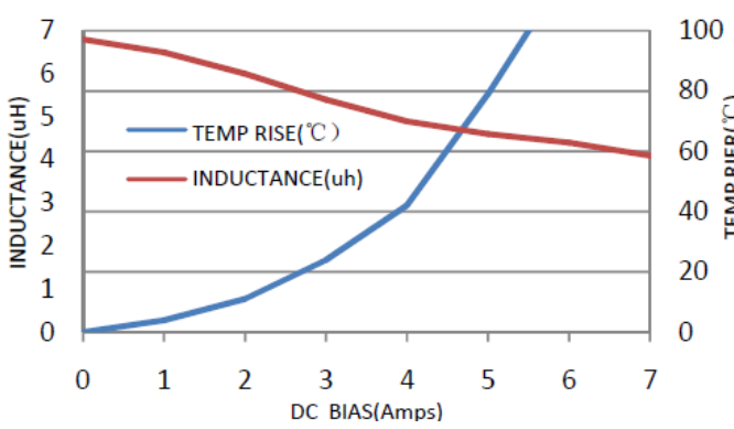
PIC05030-6R8M
