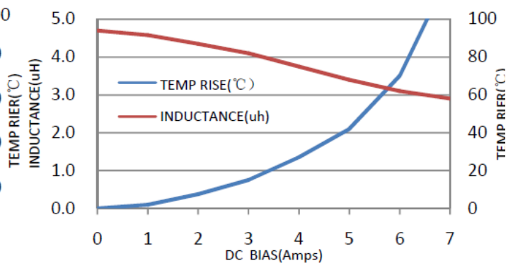
PIC05030-4R7M
