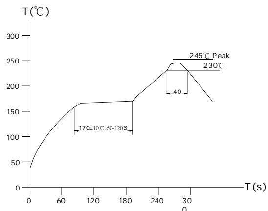
Lead-free the recommended reflow condition
