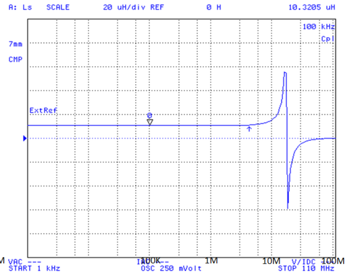
PI07018-100M
