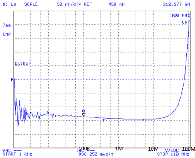
PI07018-R82M
