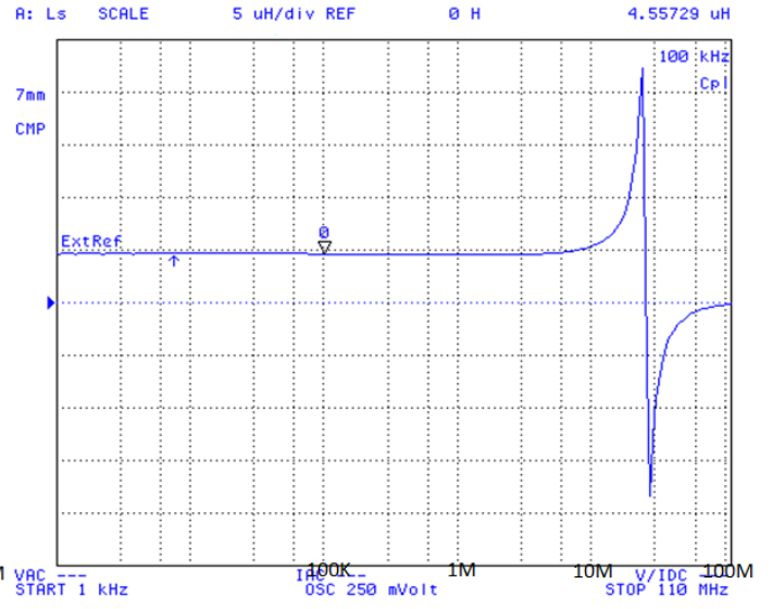
PI07018-4R7M
