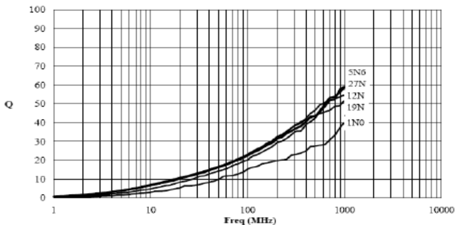
Q VS FREQUENCY
