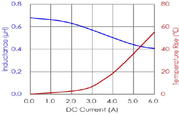
PIC252012-R68
